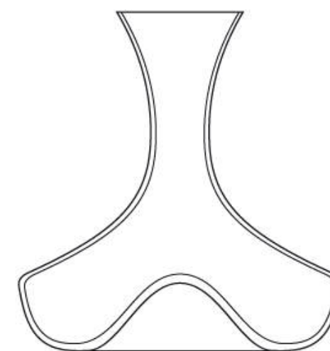
Casiopeia 1500 ml Ø 220 × H 231 mm
